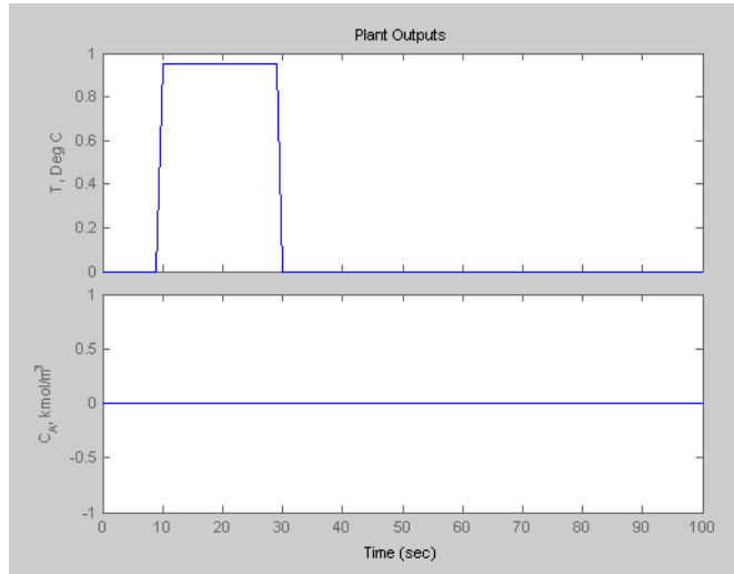
Response Plot Showing Open-Loop Pulse Disturbance
