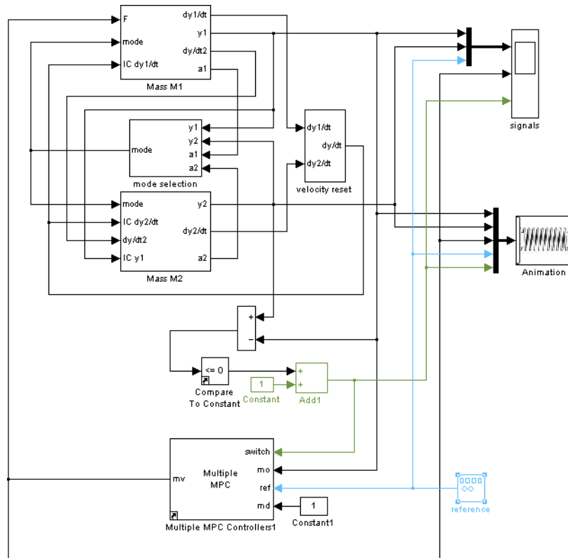
Block Diagram of the Two-Model Example
